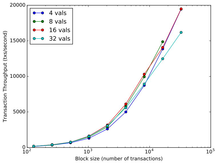
Figure 9.3: Large machines. With 32 vCPU and 60 GB of RAM, transaction throughput increases linearly with block-size, relieving the capacity limits found on smaller machines.
