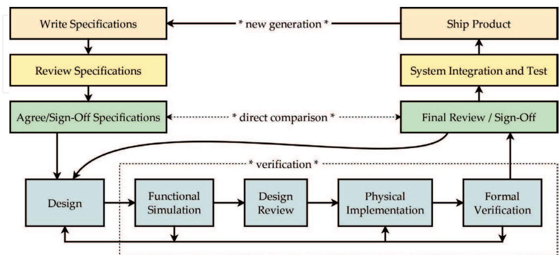
Figure 1. The universal design methodology (UDM), with an emphasis on multiple sign-off processes within the design flow and functional and final design verification against agreed specifications.
